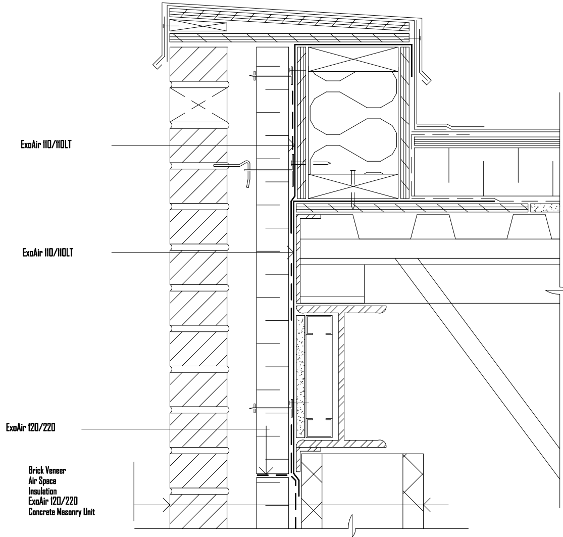
Brick Veneer/Conc. Blk. Wall
