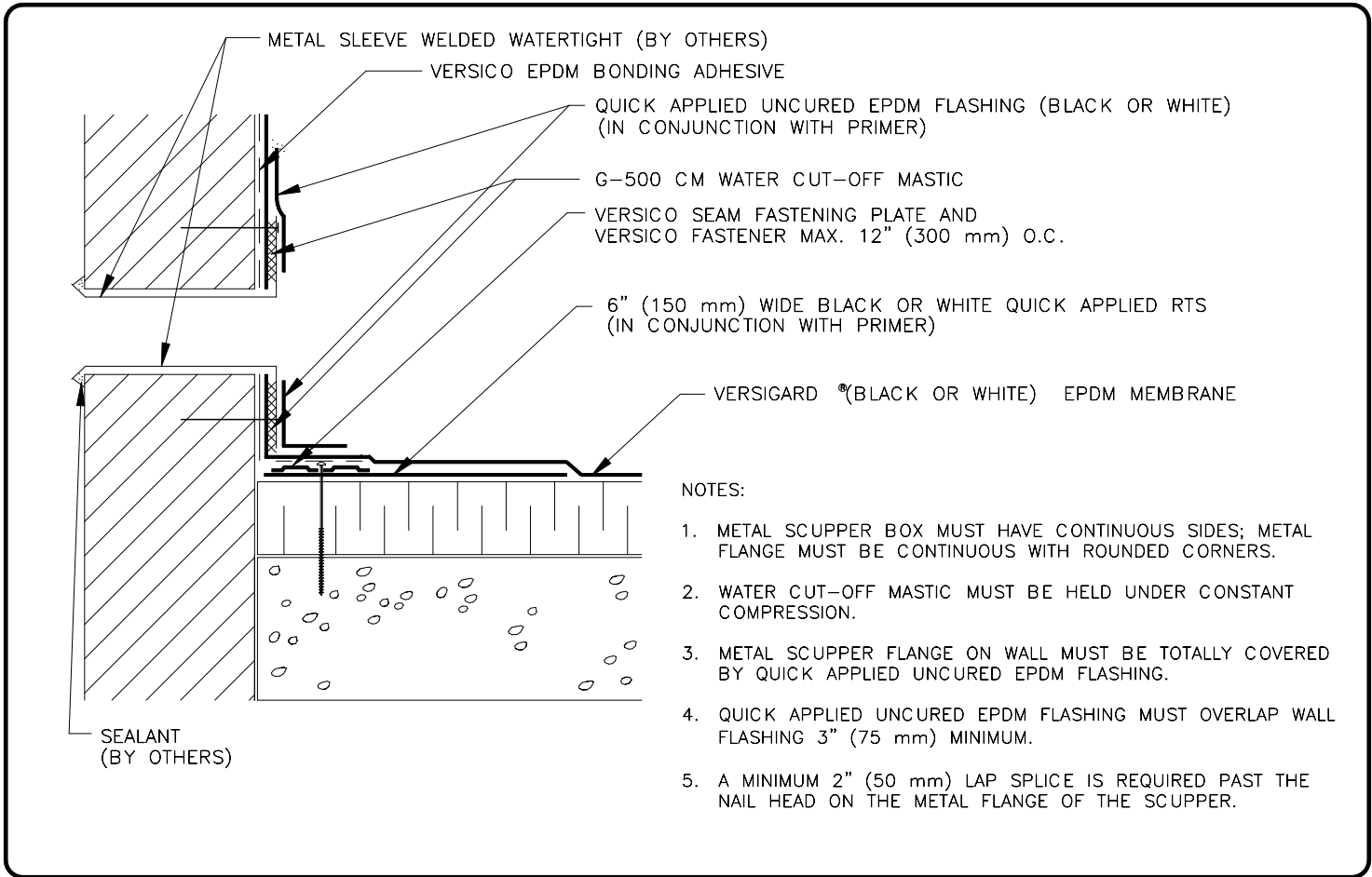
C-18.3 OVERFLOW METAL SCUPPER
