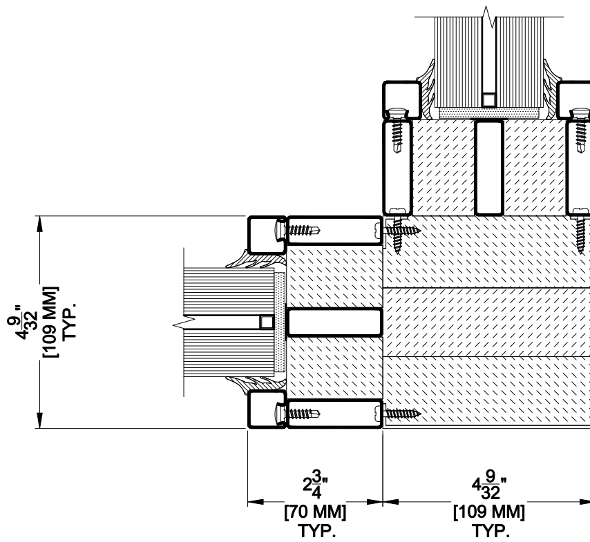
VDS-120 90° CORNER
