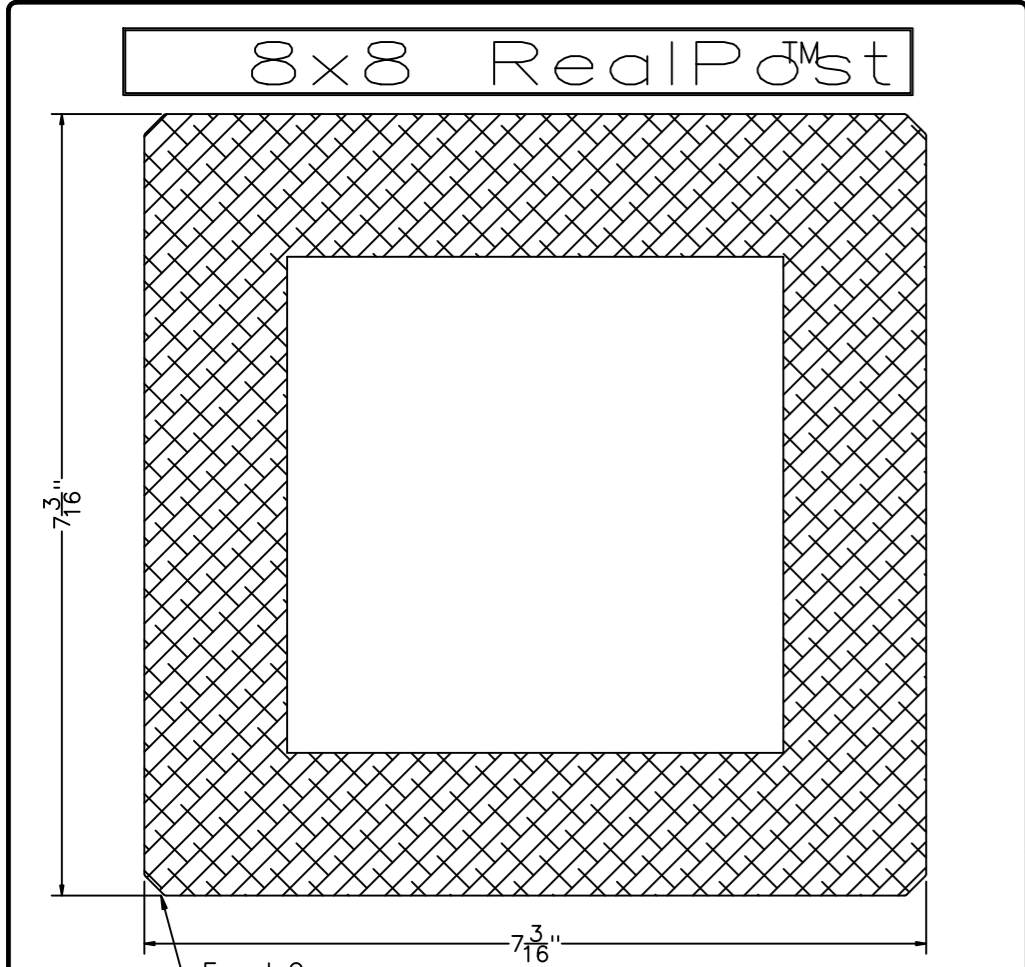
Typical Section View Full Scale
