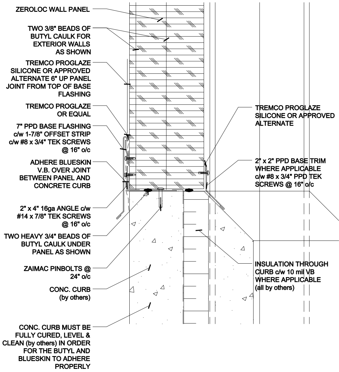
BASE OF EXTERIOR WALL PANEL ON CURB
