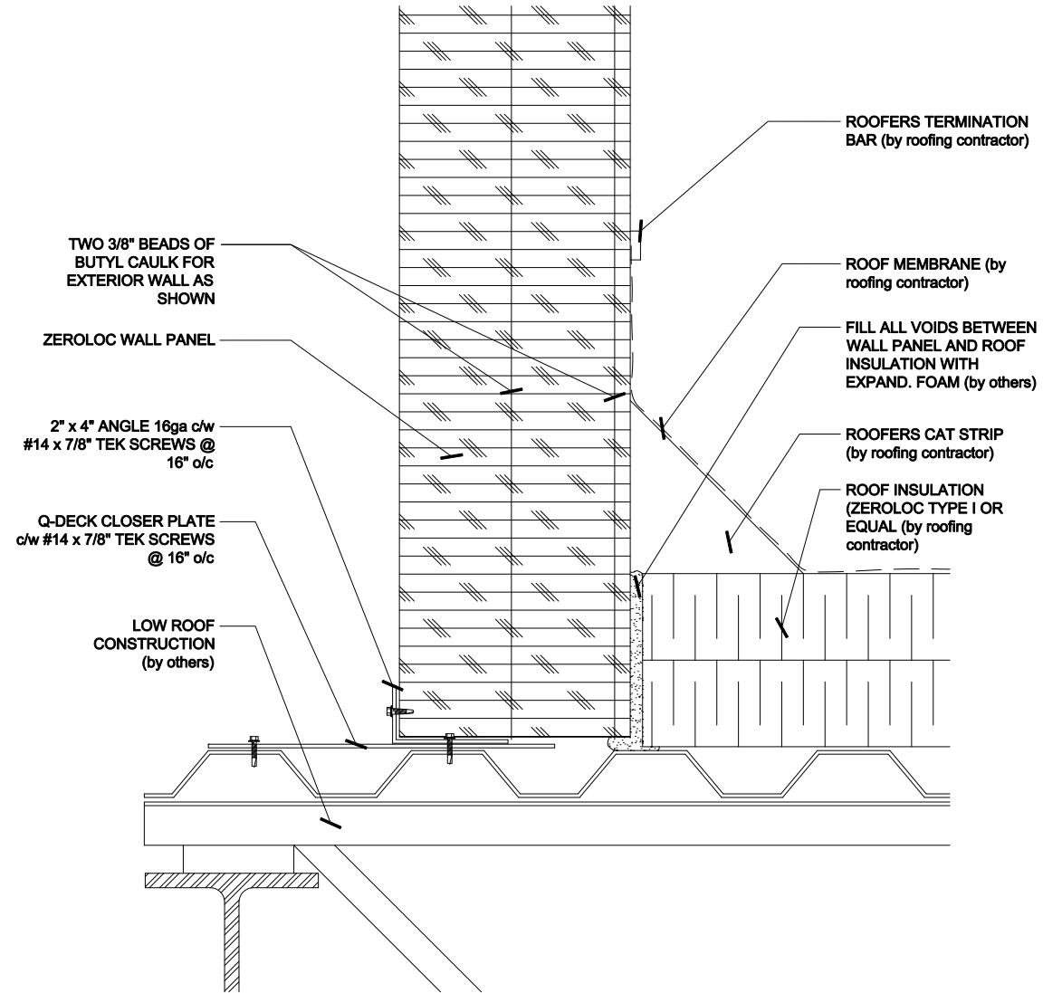
BASE OR HIGH PANEL WALL TO LOW ROOF/PENTHOUSE
