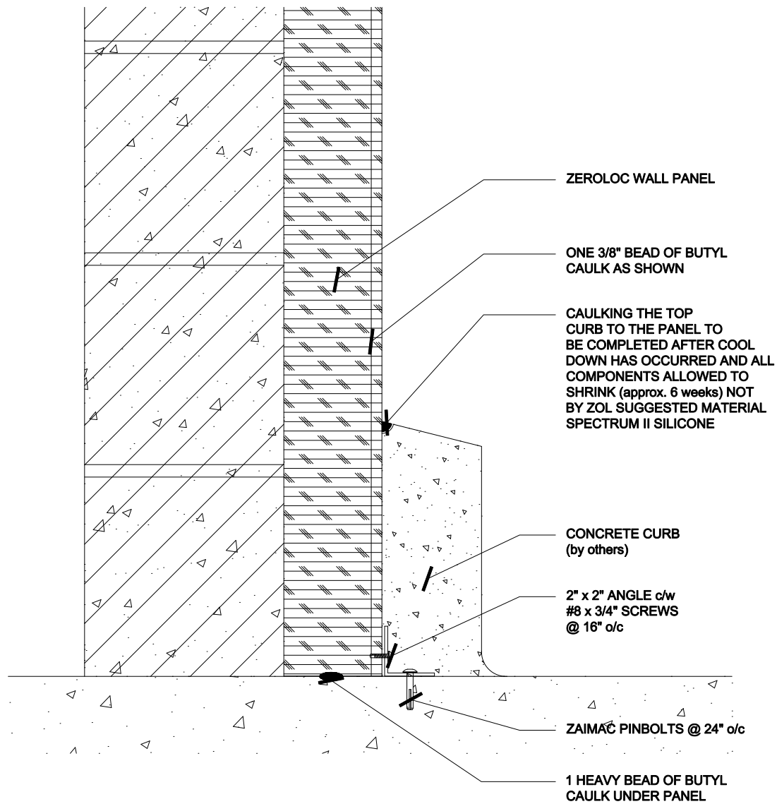
BASE OF LINER PANEL WALL
