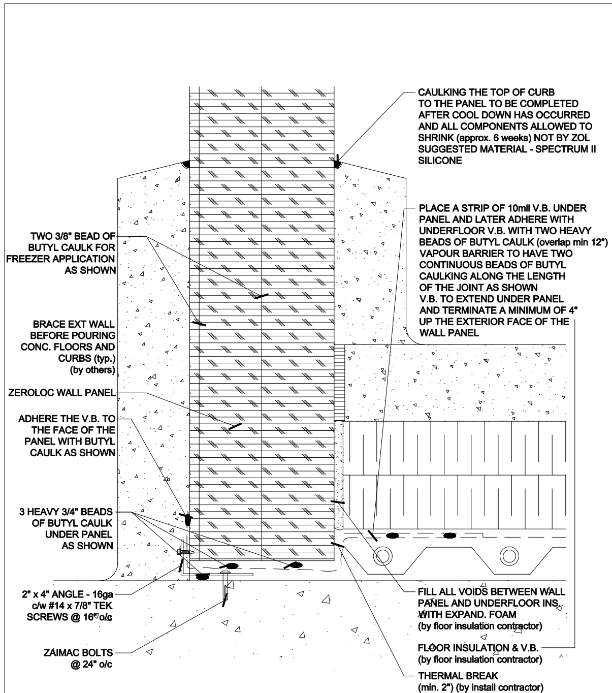
ELEVATED FREEZER FLOOR DETAIL
