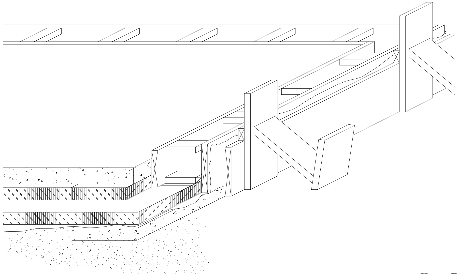
3D ILLUSTRATION OF THE RECOMMENDED BLOCK-OUT FOR DETAIL 8.02
