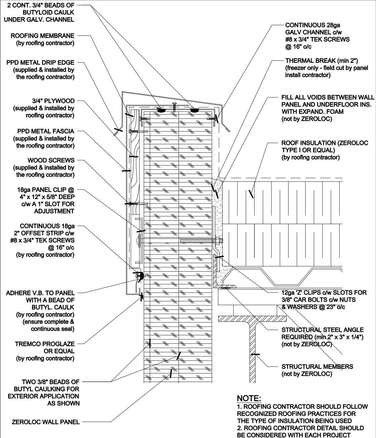
EXTERIOR TOP OF WALL WITH PARAPET
