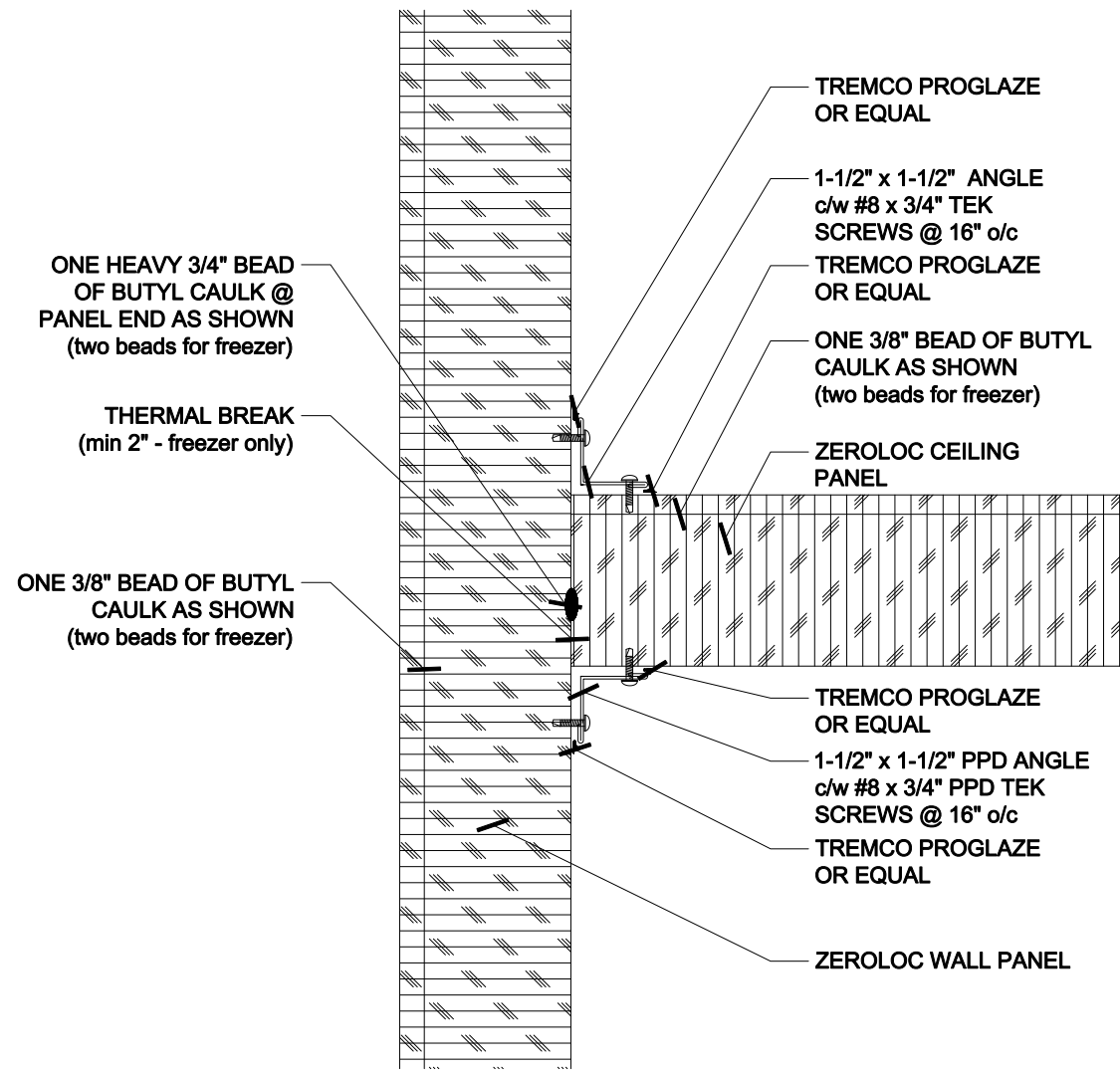
INTERIOR CEILING PANEL TO WALL DETAIL
