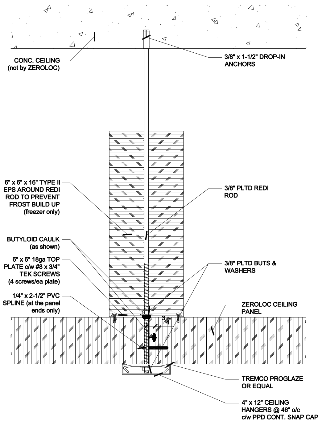
CEILING HANGER DETAIL IN CONC. DECK
