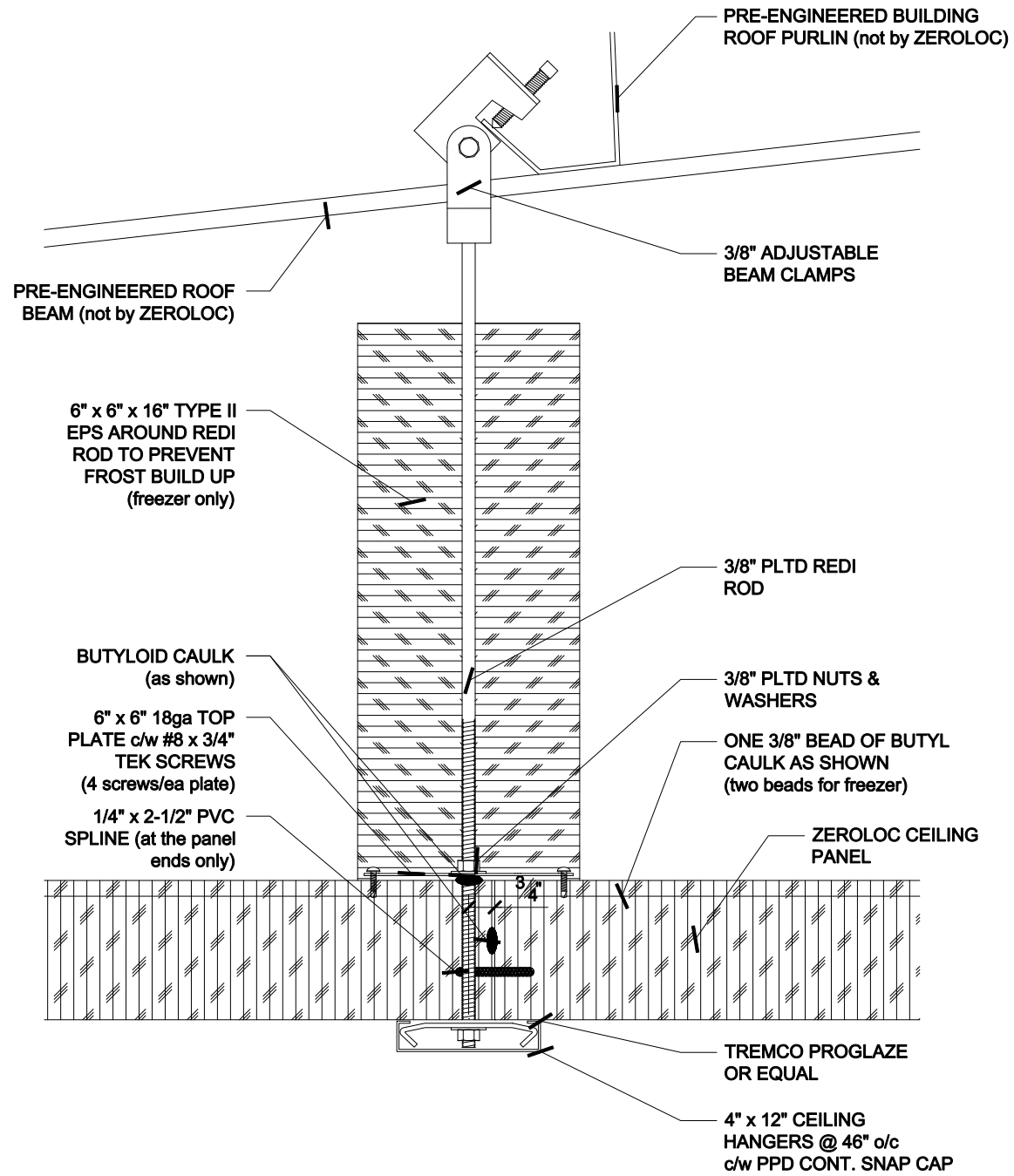
CEILING HANGER DETAIL @ PRE-ENGINEERED PURLIN
