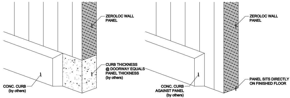
OPTION 1 PANEL SITS ON A CURB
