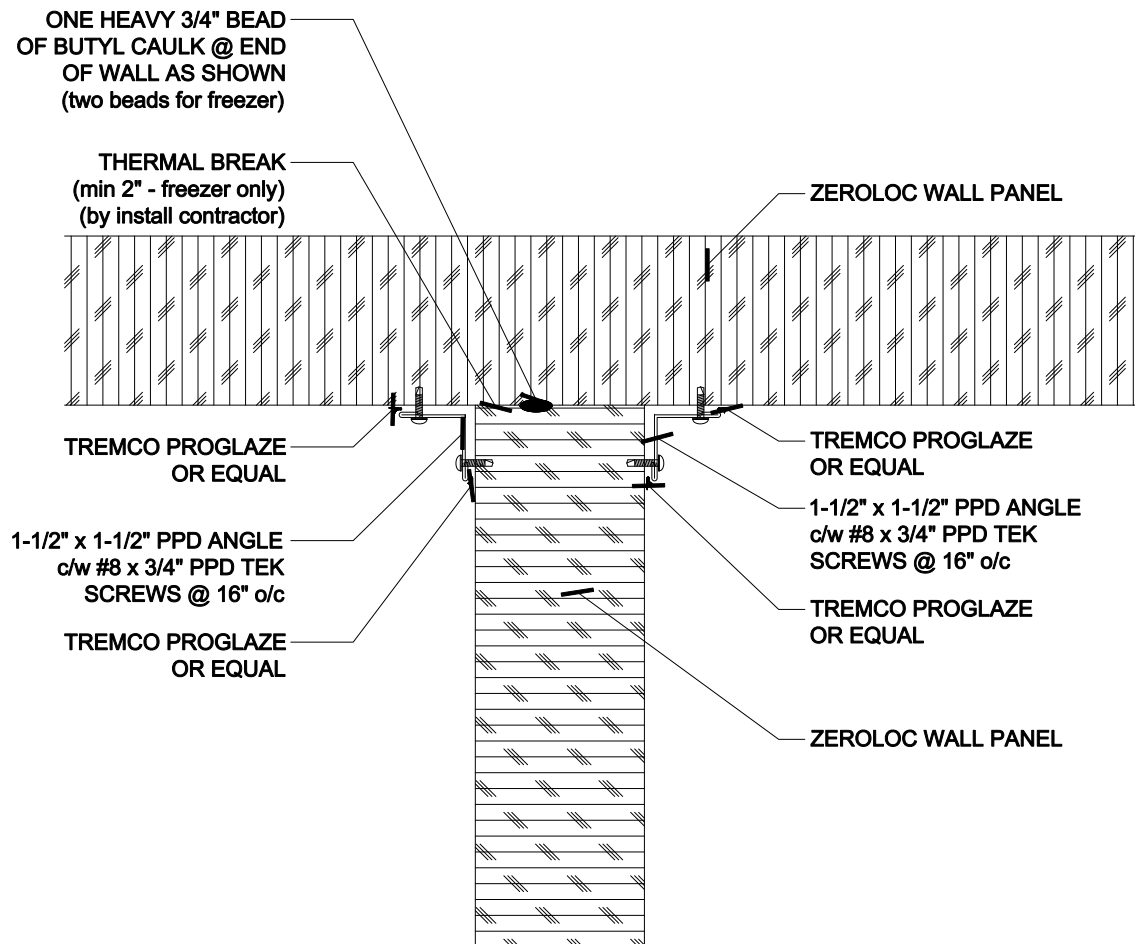
INTERIOR PARTITION WALL 'T' CONNECTION (plan view)
