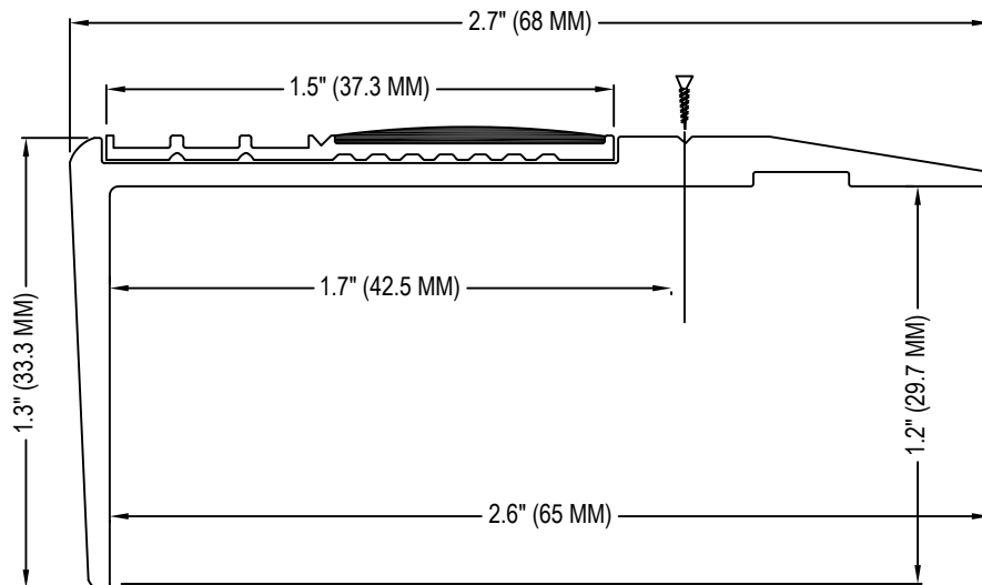
ECOGLO-PROFILE F4 SERIES FLAT NOSING
