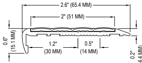
ECOGLO-PROFILE F7 SERIES WITH N SERIES INSERT
