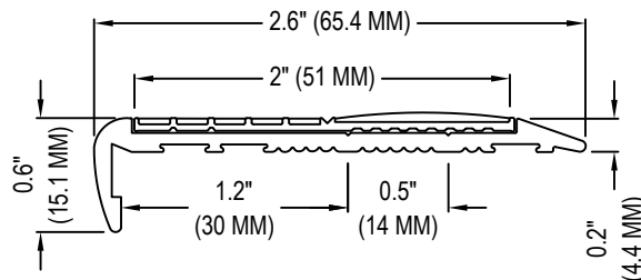
ECOGLO-PROFILE F7 SERIES WITH E40 SERIES INSERT
