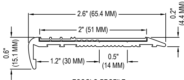
ECOGLO-PROFILE F7 SERIES WITH E30 SERIES INSERT
