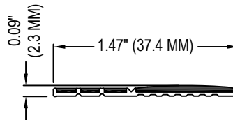
ECOGLO-PROFILE E20 SERIES NON-SLIP STRIP
