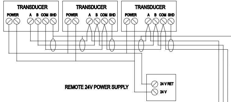
TYPICAL CONNECTION OF MRS-485
