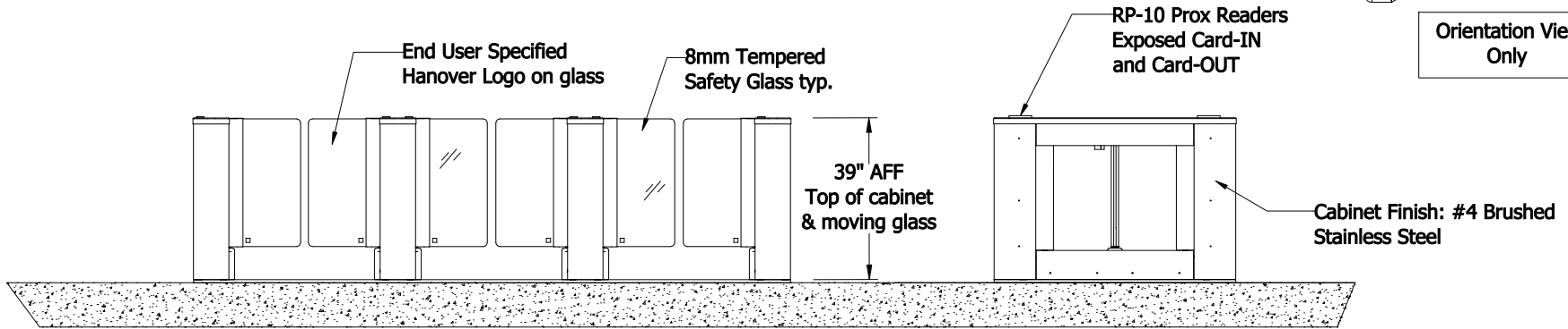
Entrance View Elevation
