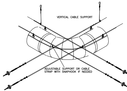
SUSPENSION DETAIL RADIUS ELBOW, 2 ROW CABLE SUSPENSION
