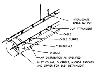
SUSPENSION DETAIL 2 ROW CABLE SUSPENSION AT 10&2 O'CLOCK
