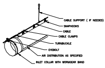
SUSPENSION DETAIL 1 ROW CABLE SUSPENSION AT 12 O'CLOCK
