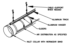
TRACK SUSPENSION DETAIL 1 ROW TRACK SUSPENSION AT 12 O'CLOCK
