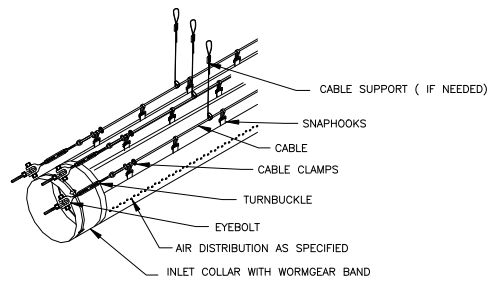
SUSPENSION DETAIL
