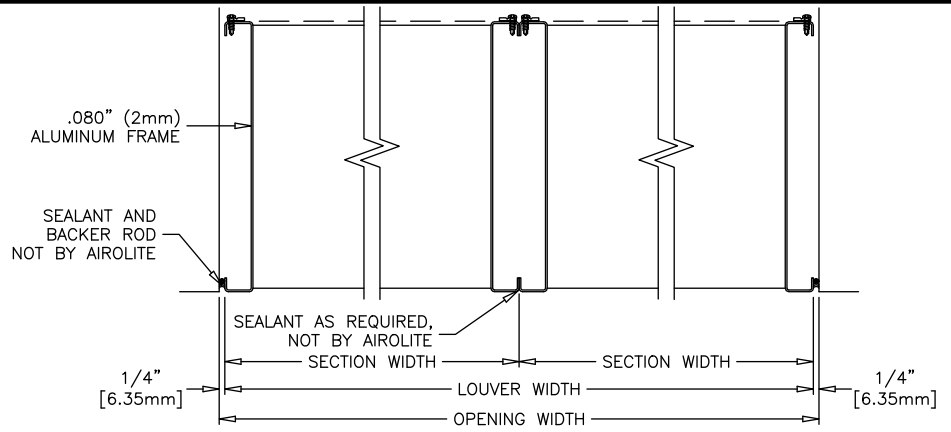
VISIBLE VERTICAL MULLION
