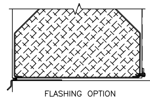
CONCEALED VERTICAL MULLION
