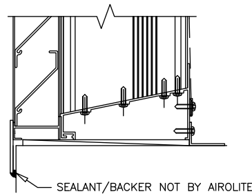
FLANGE OPTION
