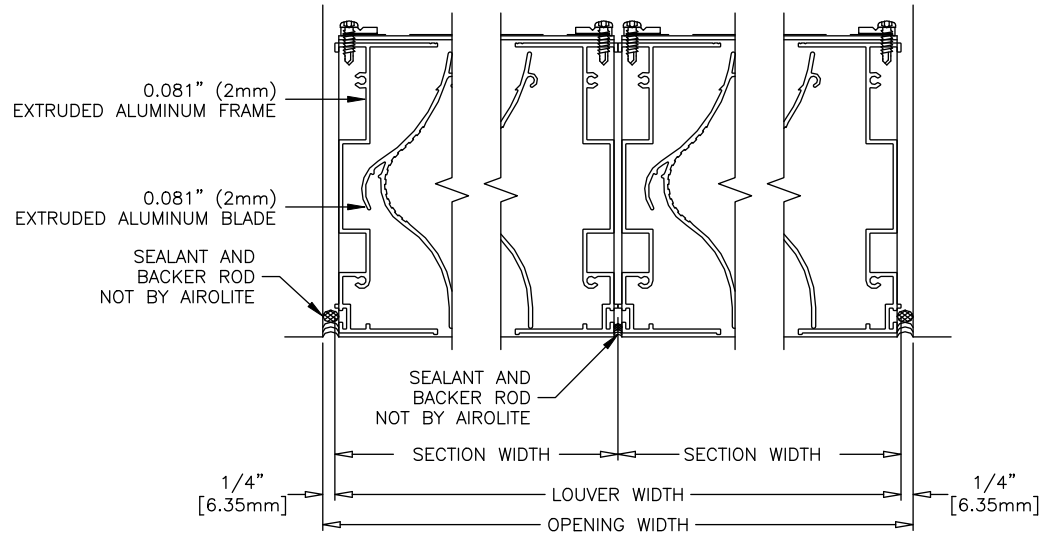
VISIBLE VERTICAL MULLION
