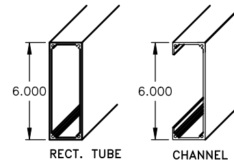
OPTIONAL FASCIA OUTRIGGER STYLE WILL VARY
