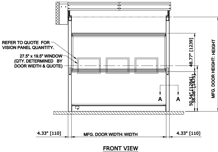
RR300-LH DOOR - WITH COVER CONTROL PANEL: CONTROLS
