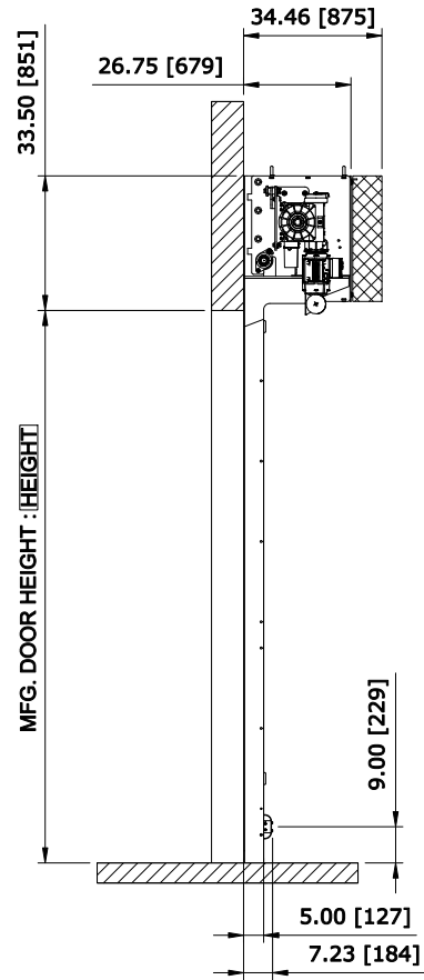
LEFT VIEW
