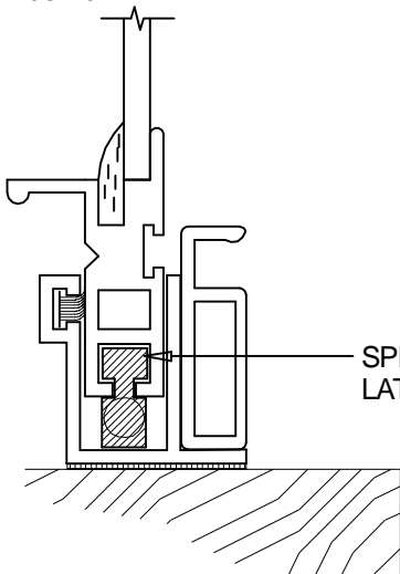
3 SILL DETAIL SCALE: FULL
