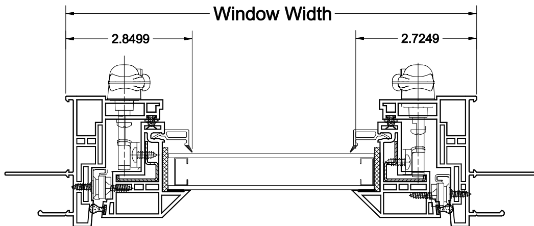
Model 0151 Single Vent Awning
