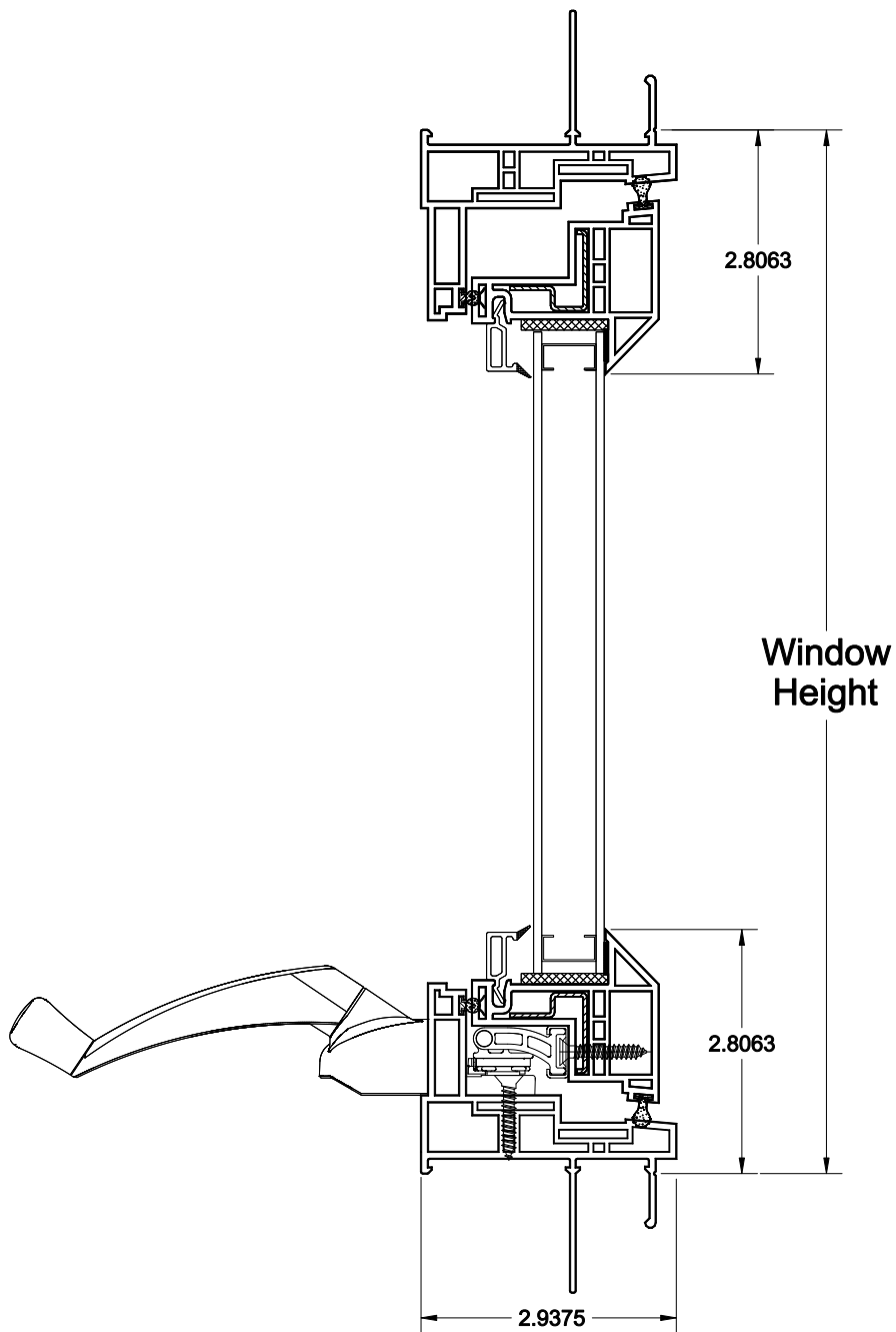
Model 0151 Single Vent Awning
