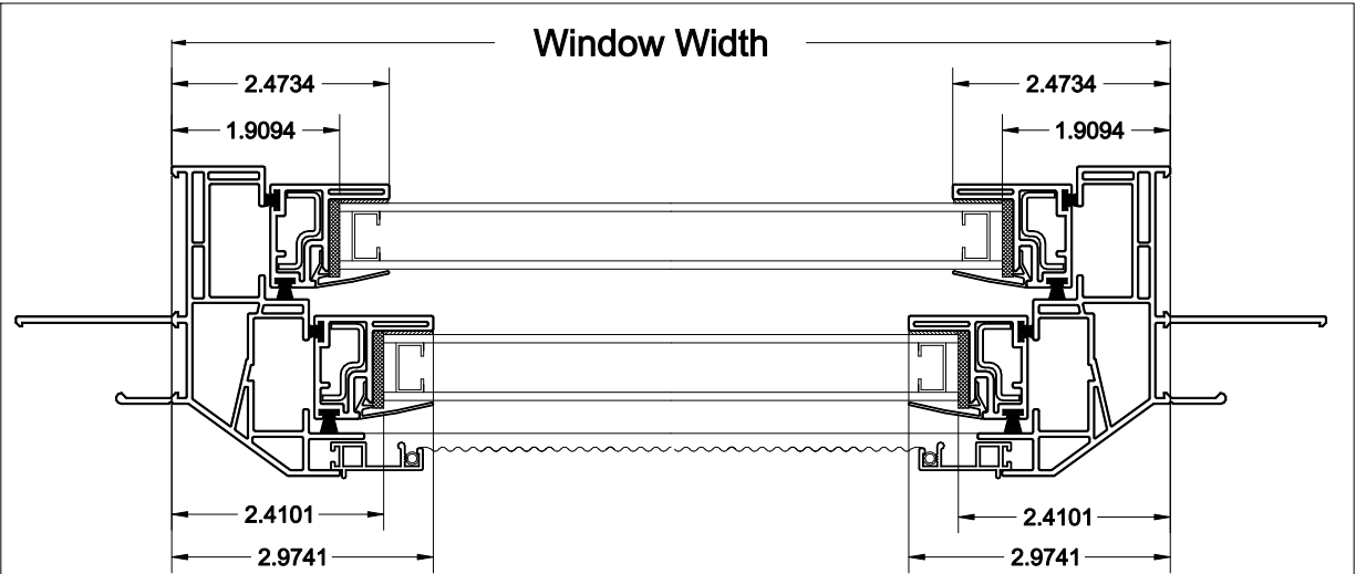
Model 0301 New Construction Double Hung
