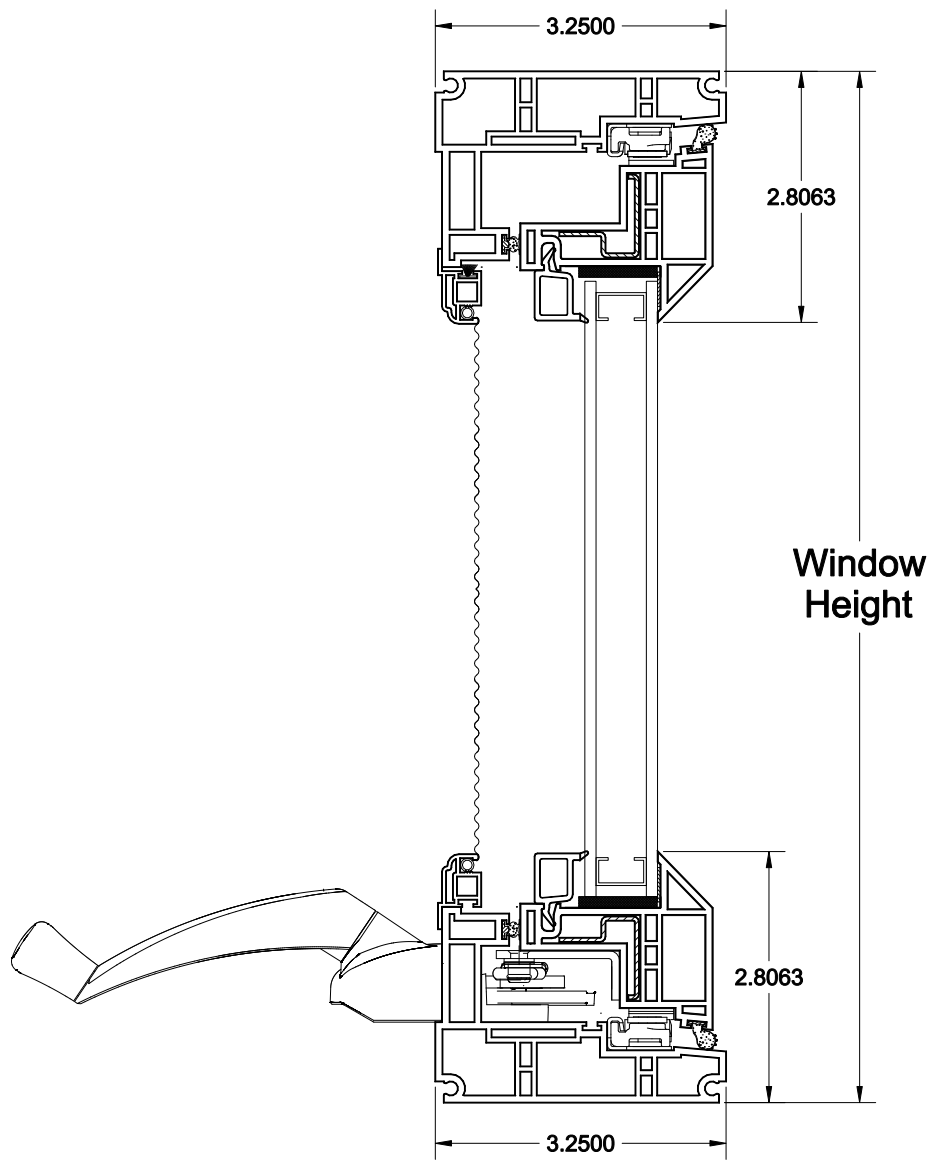
Model 0971 Single Vent Casement
