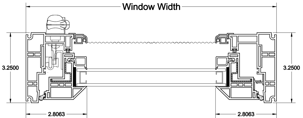
Model 0971 Single Vent Casement
