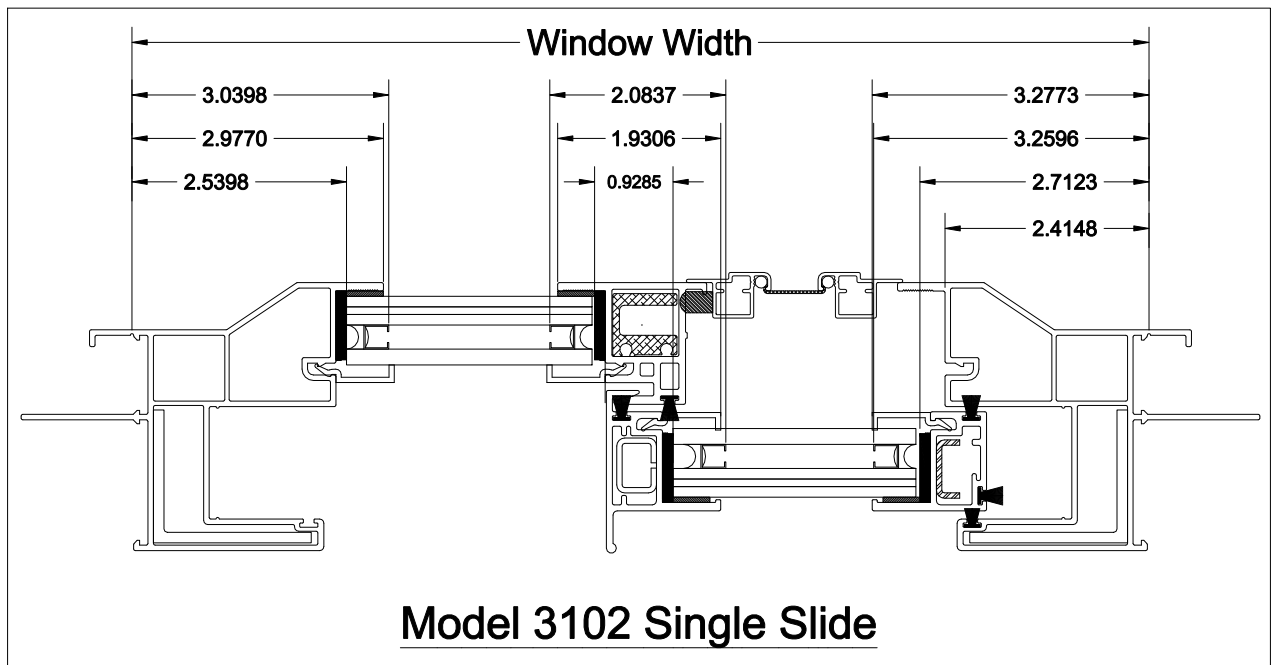
Model 3102 Single Slide
