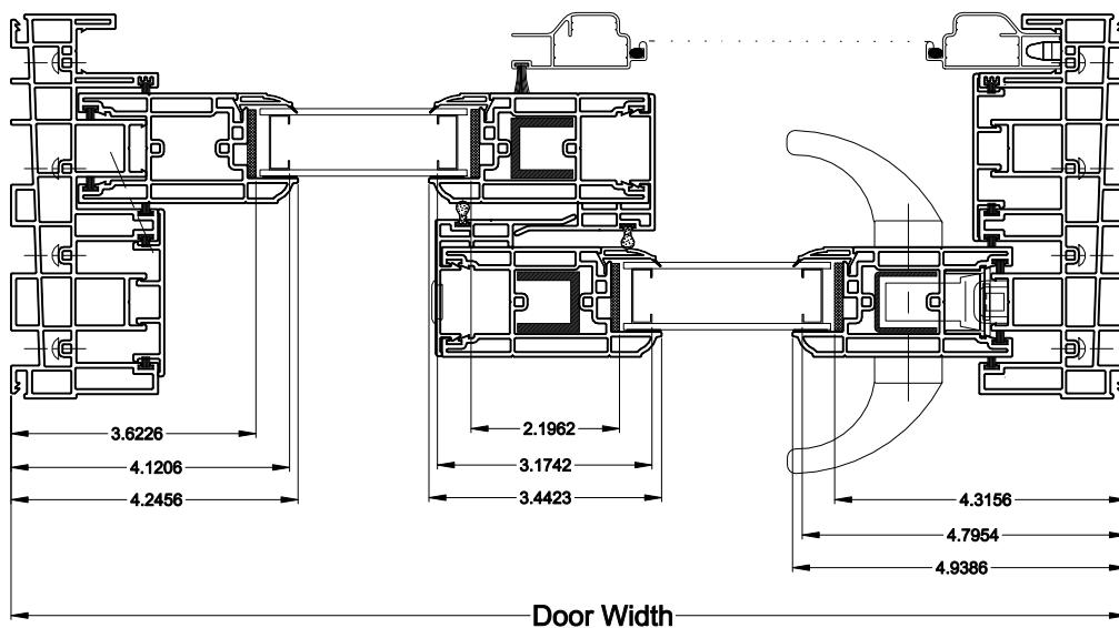
Model 6402 / 6475 French Sash Patio Door
