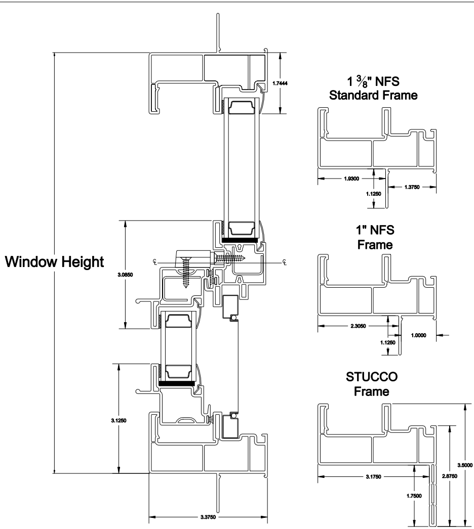
Model A581 Single Hung
