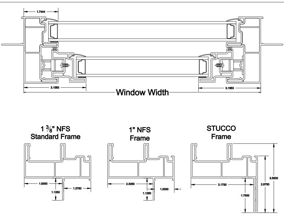
Model A581 Single Hung
