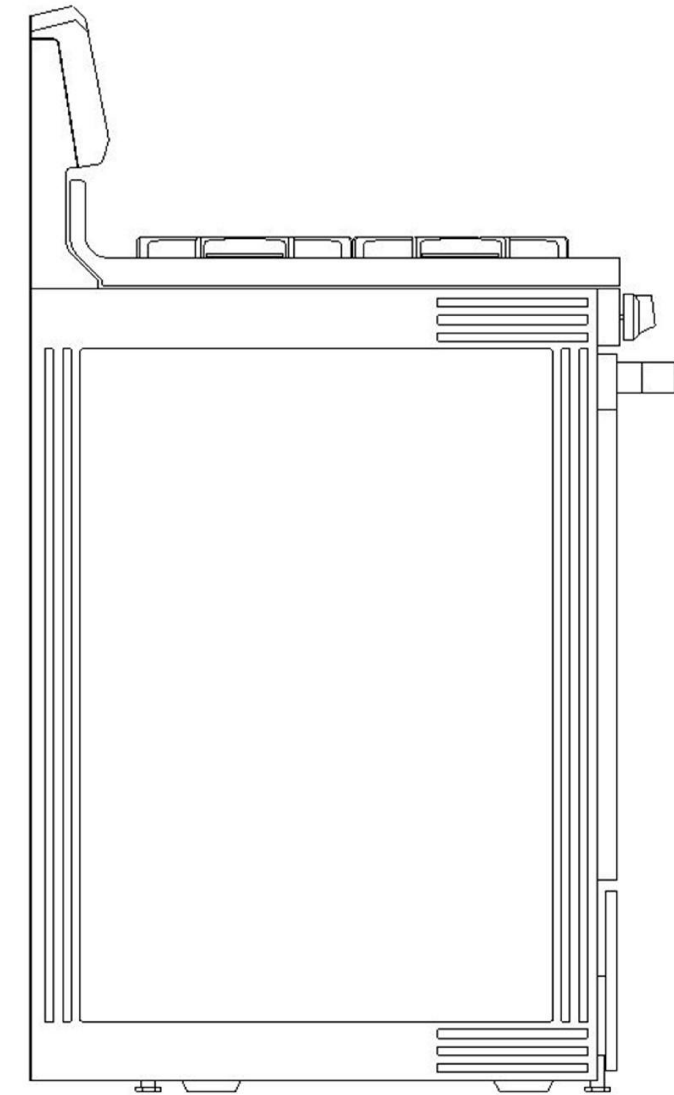
SIDE
