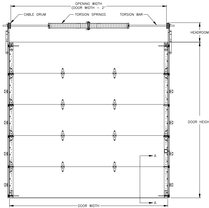
INTERIOR ELEVATION
