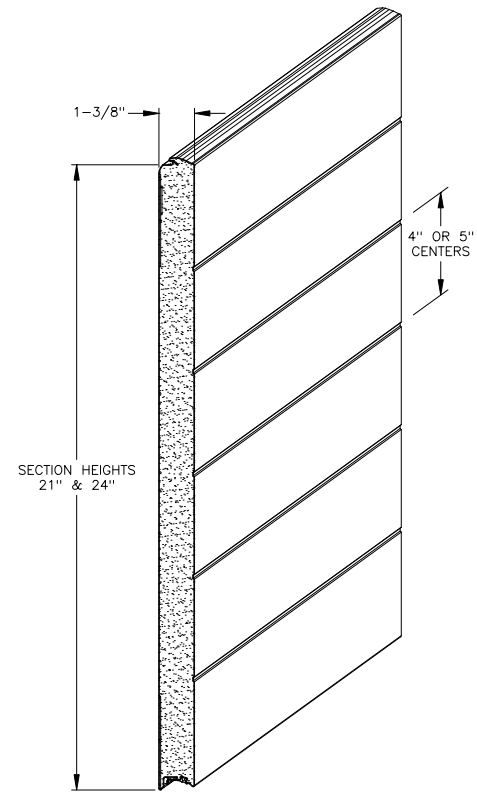
ISOMETRIC PROFILE
