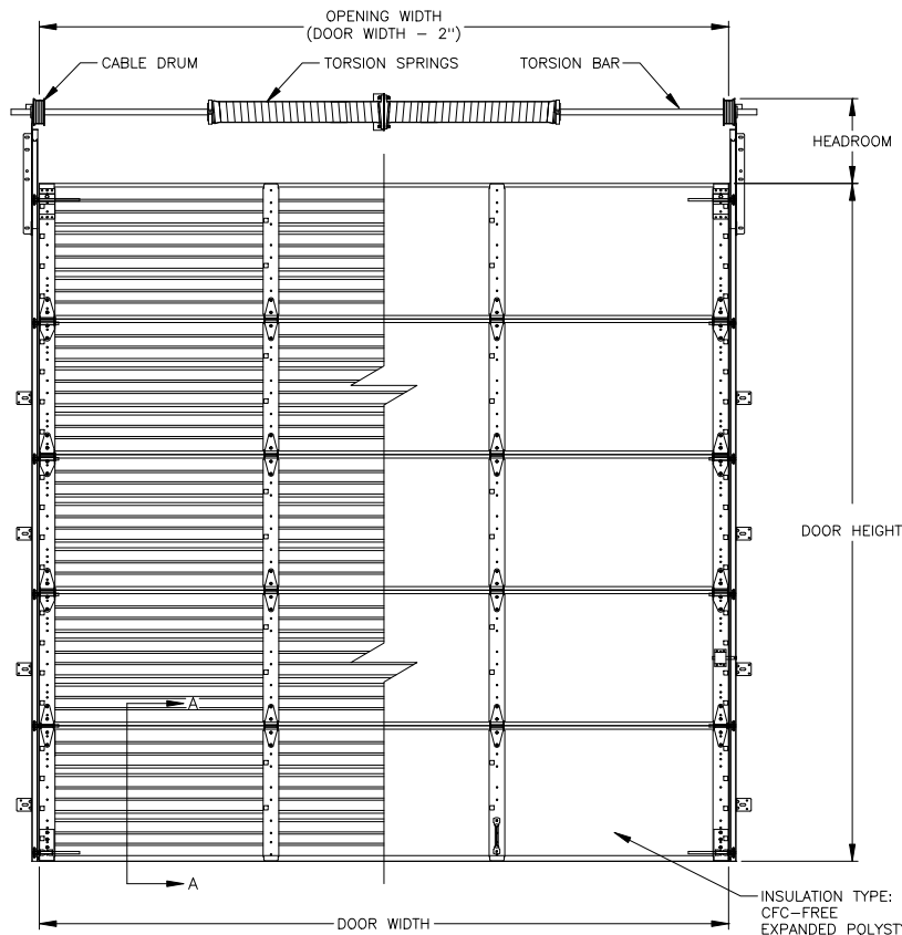
INTERIOR ELEVATION
