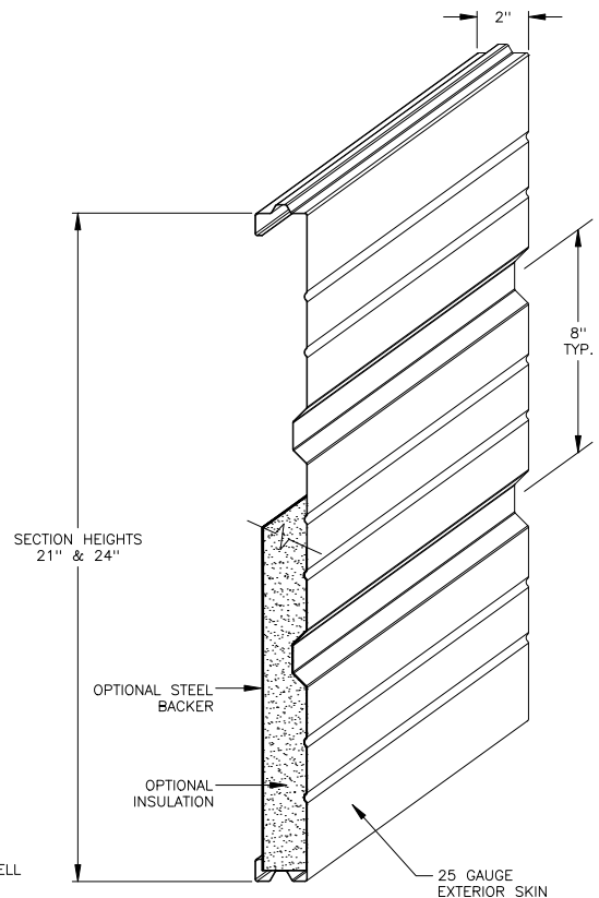
ISOMETRIC PROFILE
