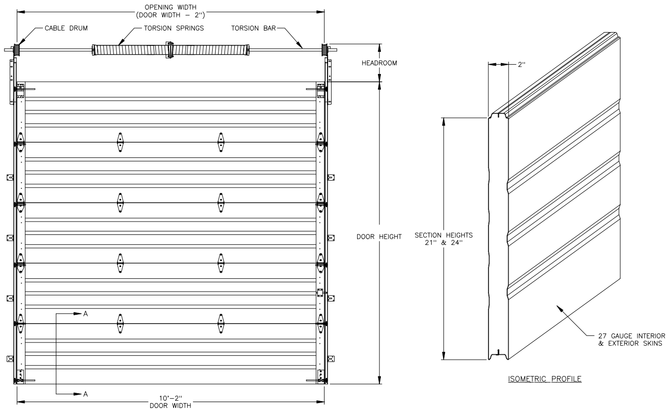
INTERIOR ELEVATION
