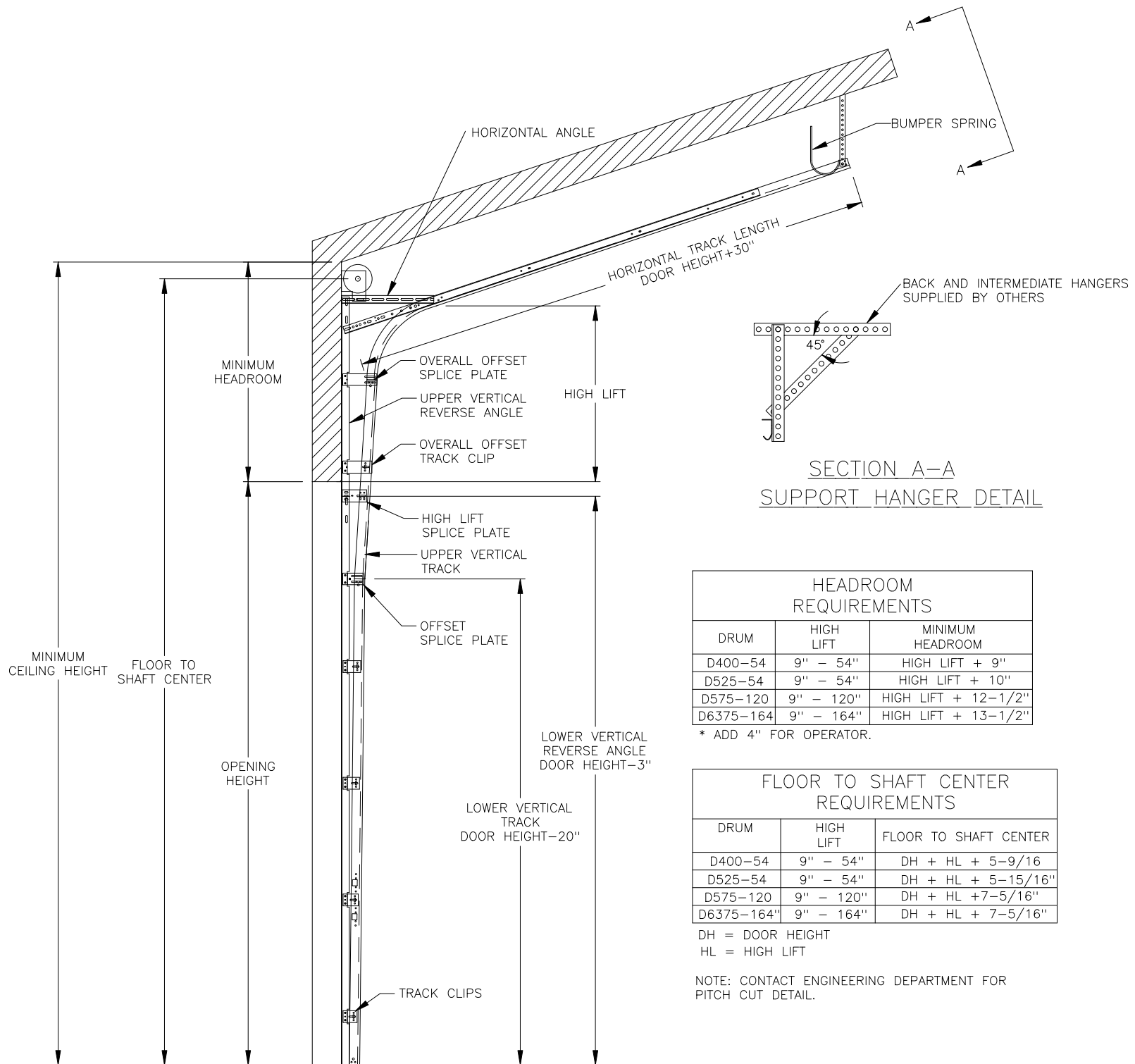
HIGH LIFT ANGLE MOUNT TRACK SET DETAIL
