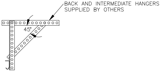
SECTION A-A SUPPORT HANGER DETAIL
