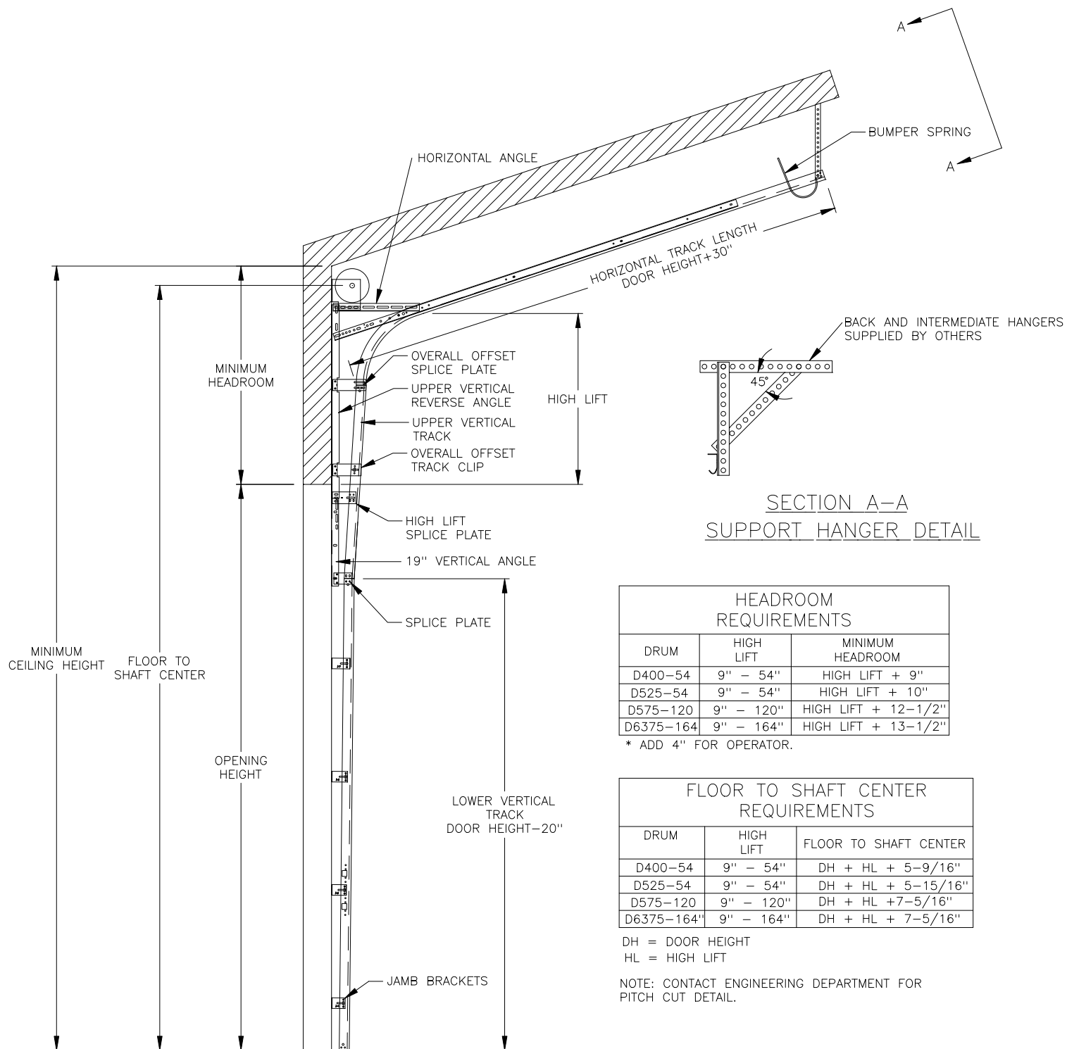
HIGH LIFT BRACKET MOUNT TRACK SET DETAIL
