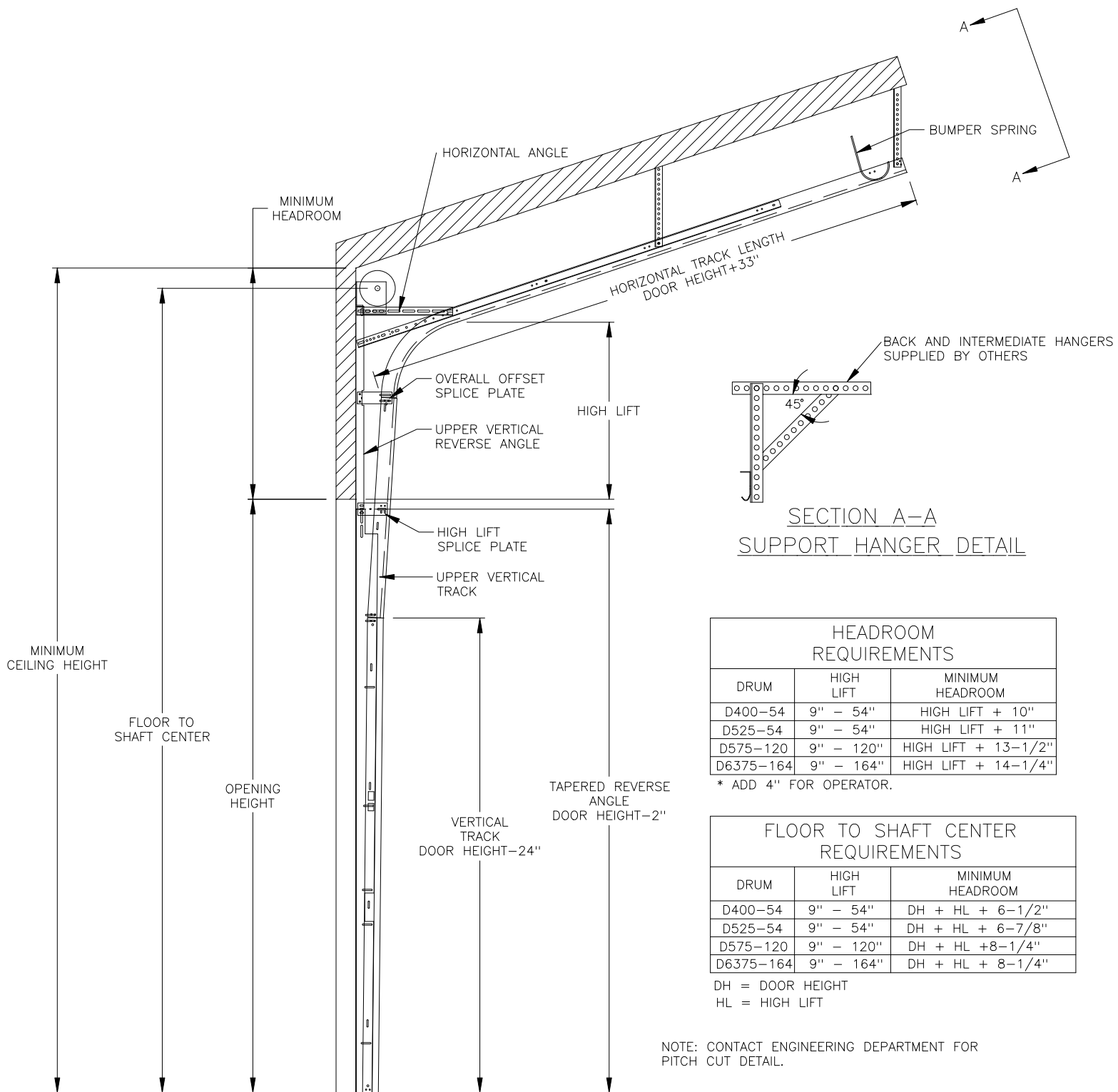
HIGH LIFT TAPERED REVERSE ANGLE MOUNT TRACK SET DETAIL
