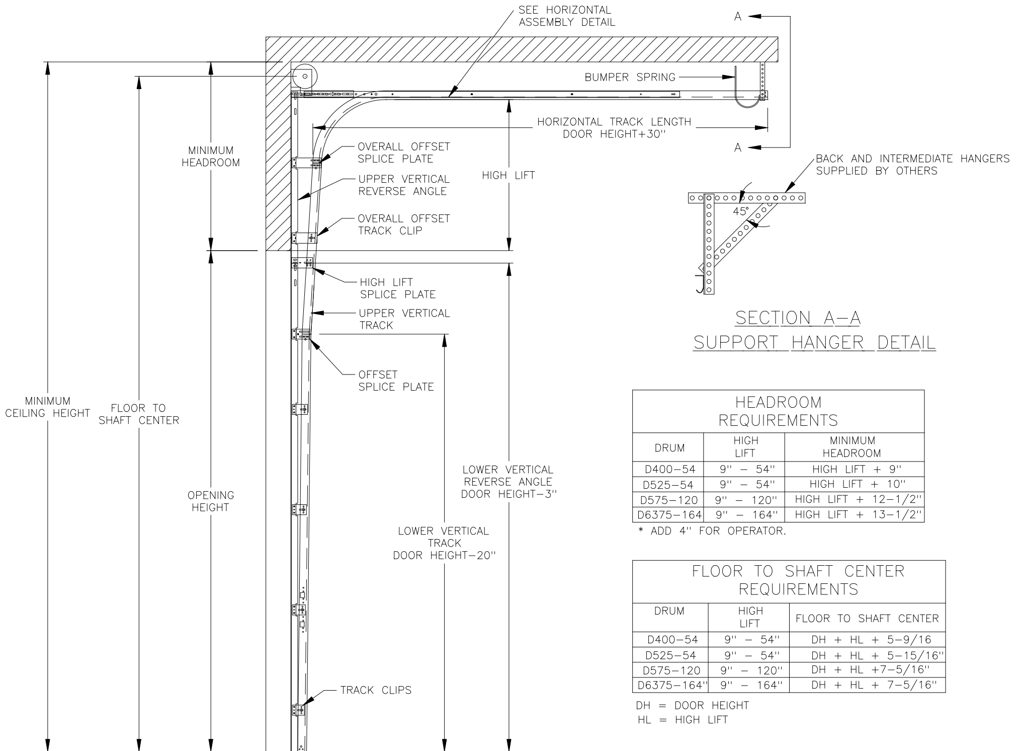
HIGH LIFT ANGLE MOUNT TRACK SET DETAIL
