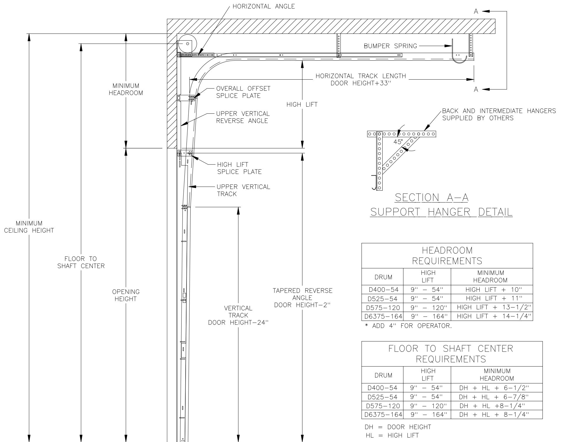
HIGH LIFT TAPERED REVERSE ANGLE MOUNT TRACK SET DETAIL
