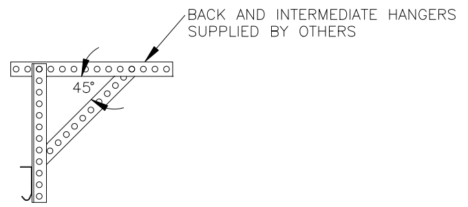
SECTION A-A SUPPORT HANGER DETAIL
