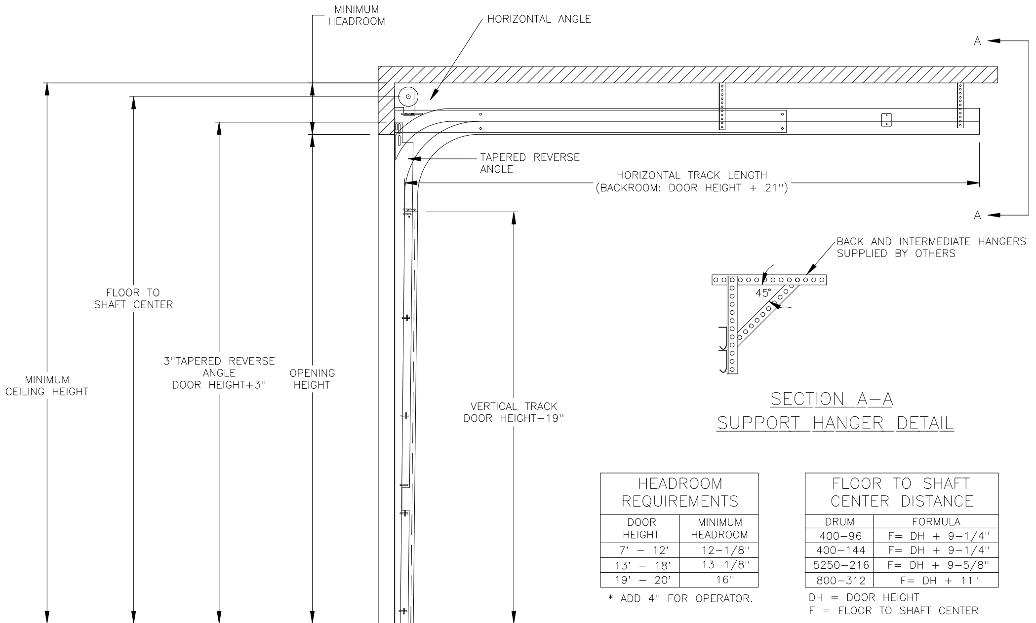
STANDARD LIFT LOW HEADROOM TO THE FRONT TAPERED REVERSE ANGLE MOUNT TRACK SET DETAIL
