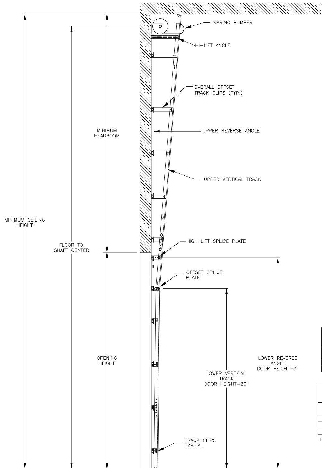
VERTICAL LIFT ANGLE MOUNT TRACK SET DETAIL
