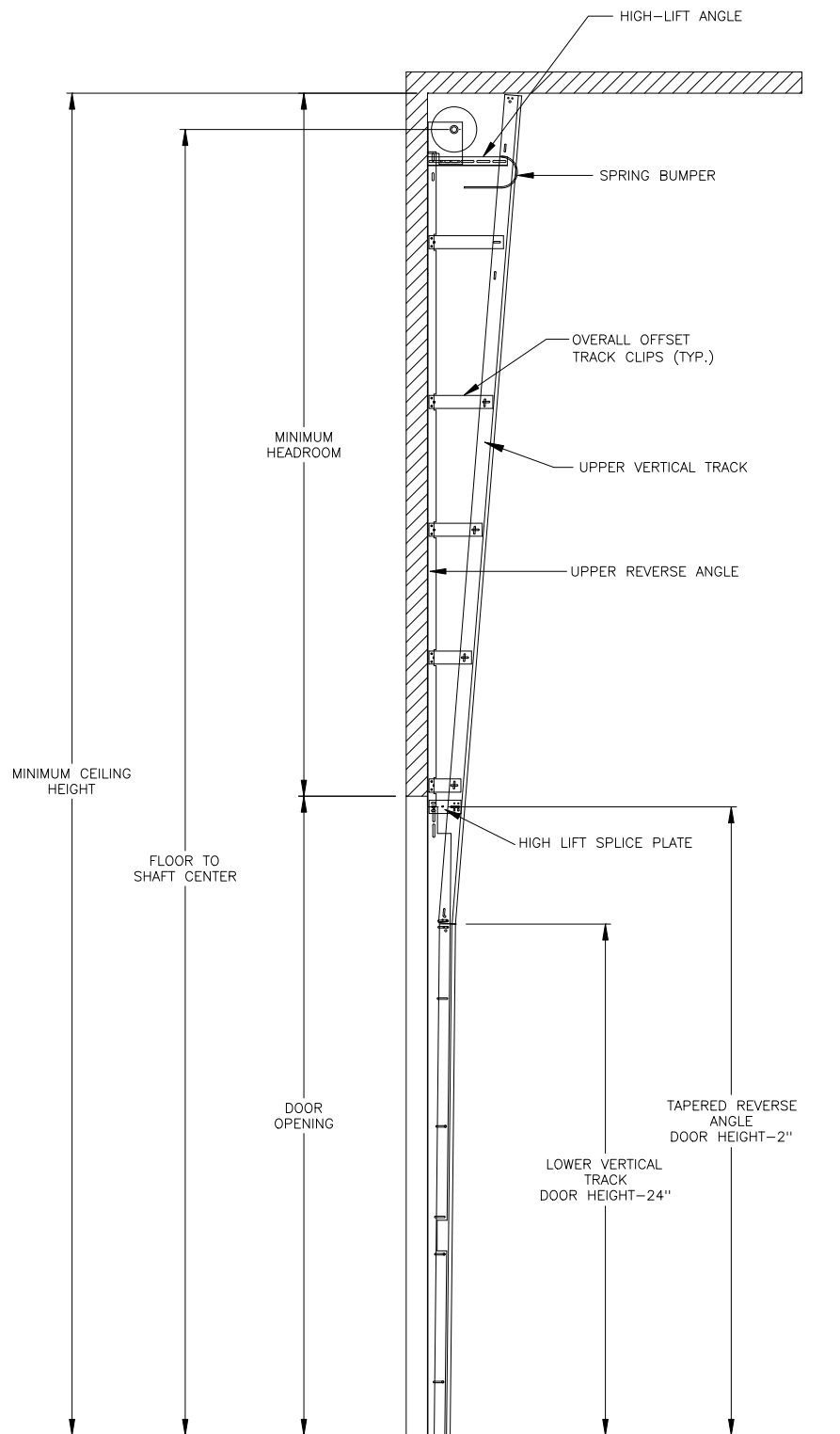
VERTICAL LIFT TAPERED REVERSE ANGLE MOUNT TRACK SET DETAIL
